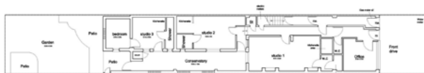
Existing ground floor plan ( Not to Scale )
